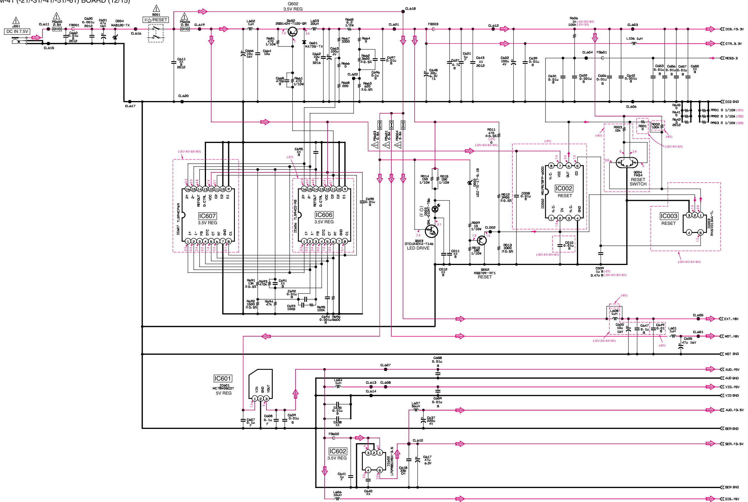
PM-41 (-21/-31/-41/-51/-61) BOARD (12/15)
