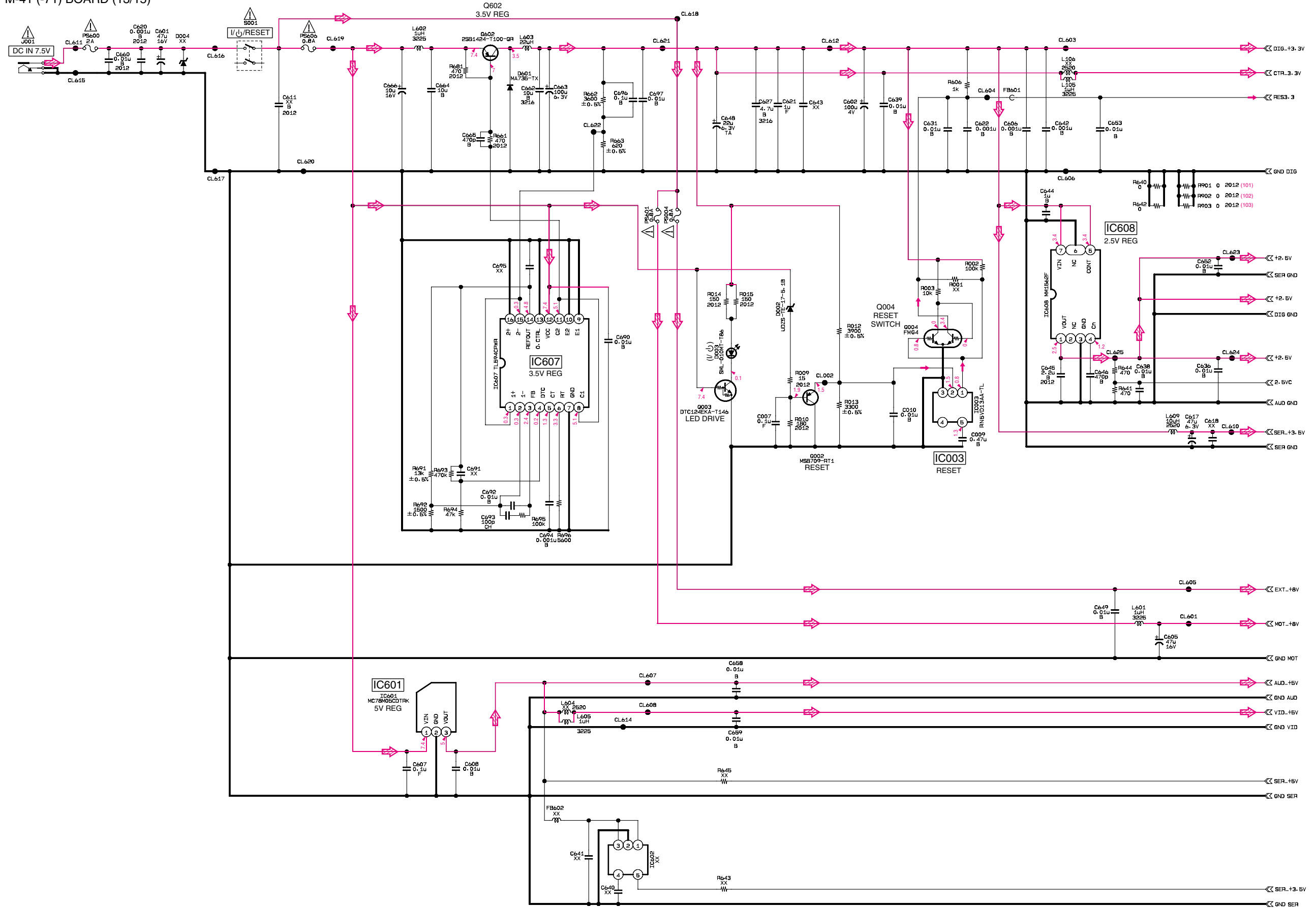
PM-41 (-71) BOARD (13/15)
