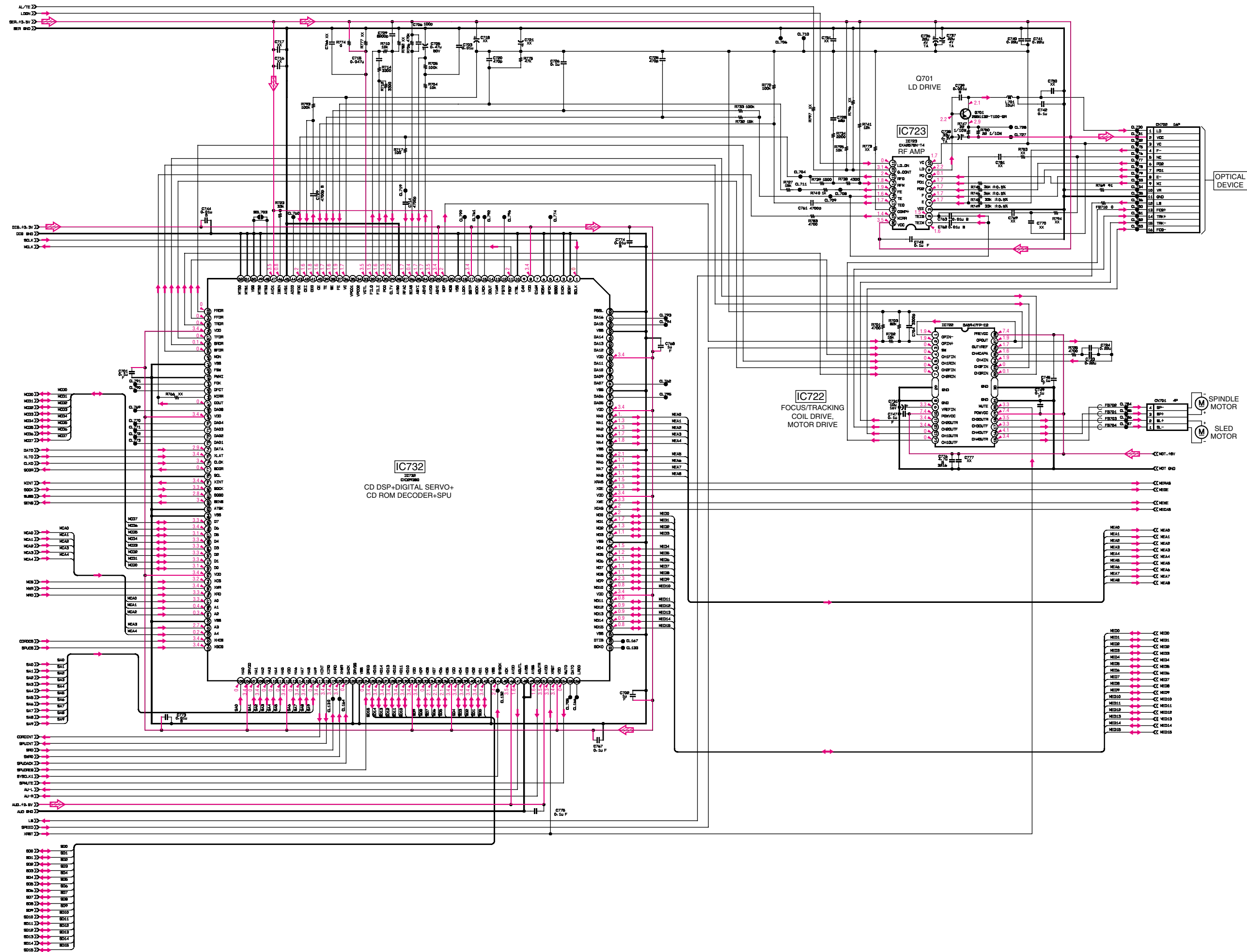
PM-41 (-11/-21/-31/-41/-51/-61) BOARD (14/15)
